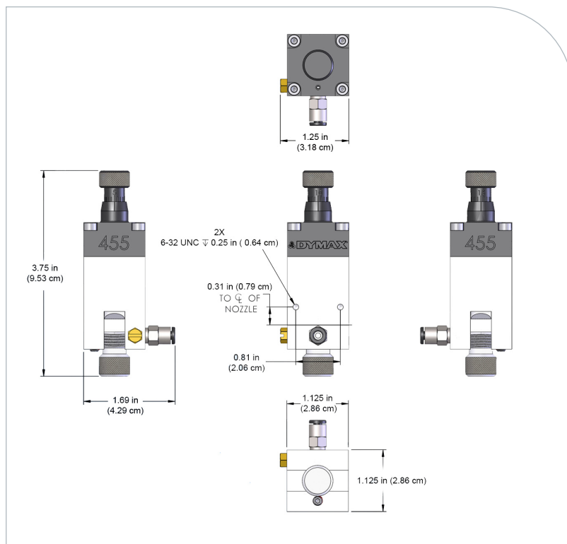
Figure 1. Model 455 Dimensions
